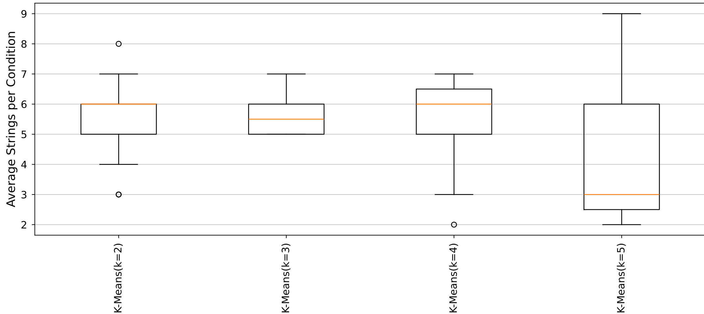
YARA Rules Average Strings per Condition Distribution (Cluster38_Size5 dataset)
